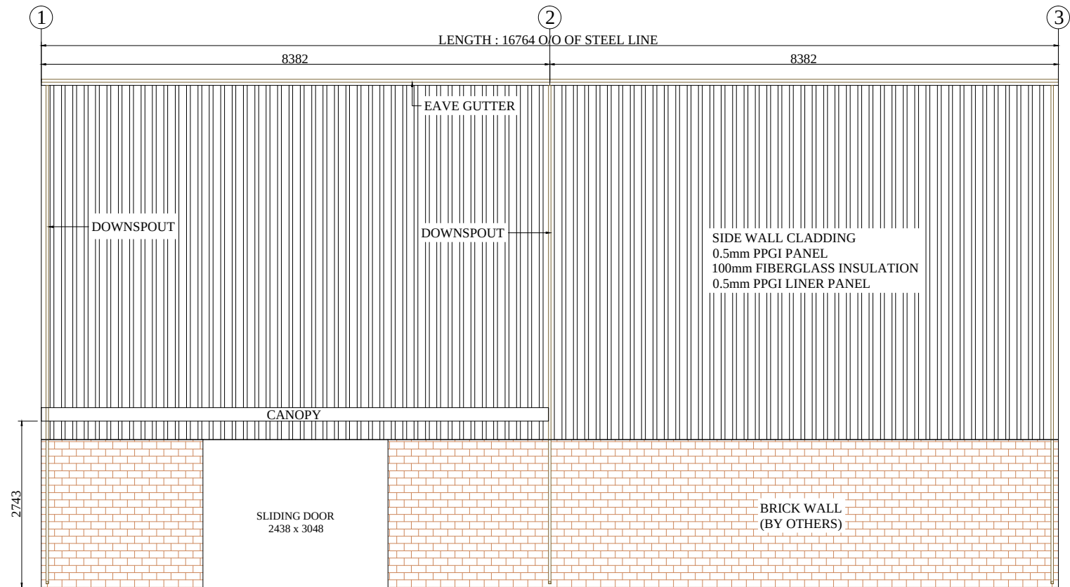
SIDE WALL ELEVATION @ GRID - A
